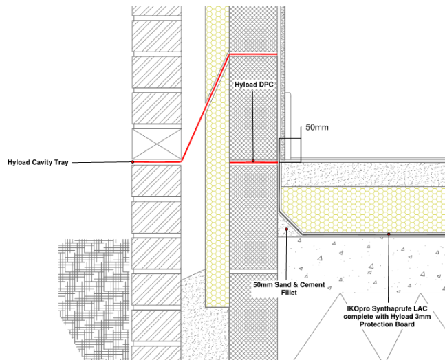
Figure 2 - Junction with a pre-existing floor and wall DPC
