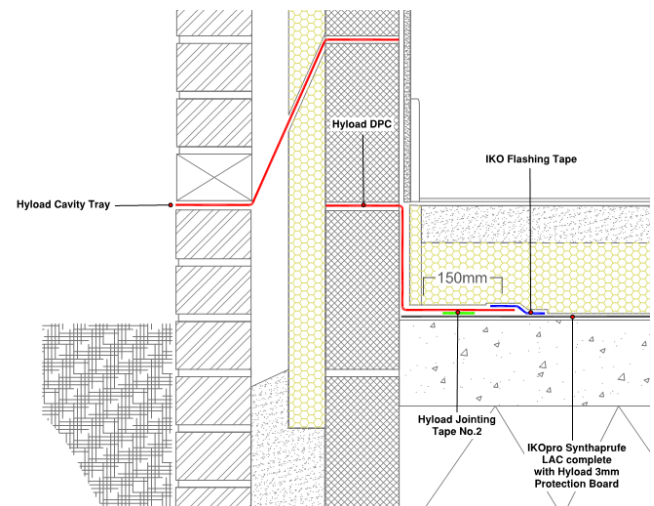
Figure 1 - Perimeter lap arrangement with DPC
